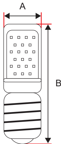
Front View
